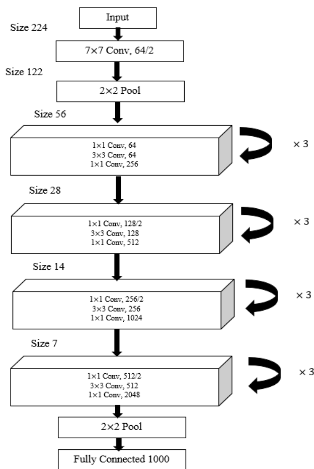
Figure. 3 Resnet 50 architecture
