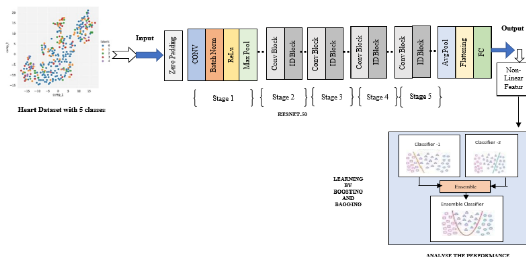
Figure. 1 Proposed Architecture
